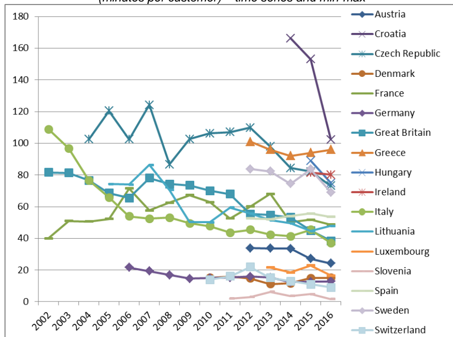
Figure 4 – Electricity: unplanned SAIDI, without exceptional events, only countries not exceeding 200 minutes
