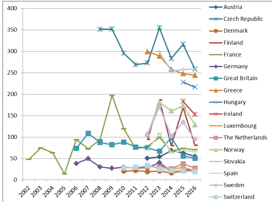
Figure 8 – Electricity: planned and unplanned SAIDI, including exceptional events, only countries not exceeding 400 minutes (minutes per customer) – time series and min-max
