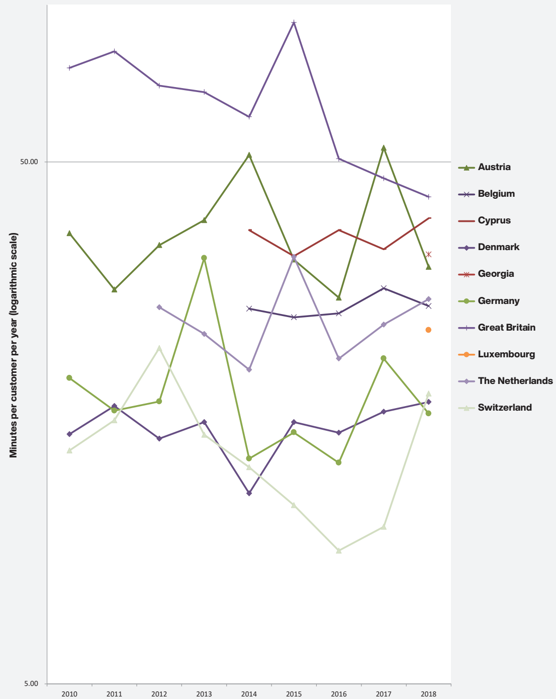
FIGURE 2-10: Unplanned long interruptions, SAIDI, all events (minutes per customer per year) – countries not exceeding 100 minutes in any of the years in the time series
