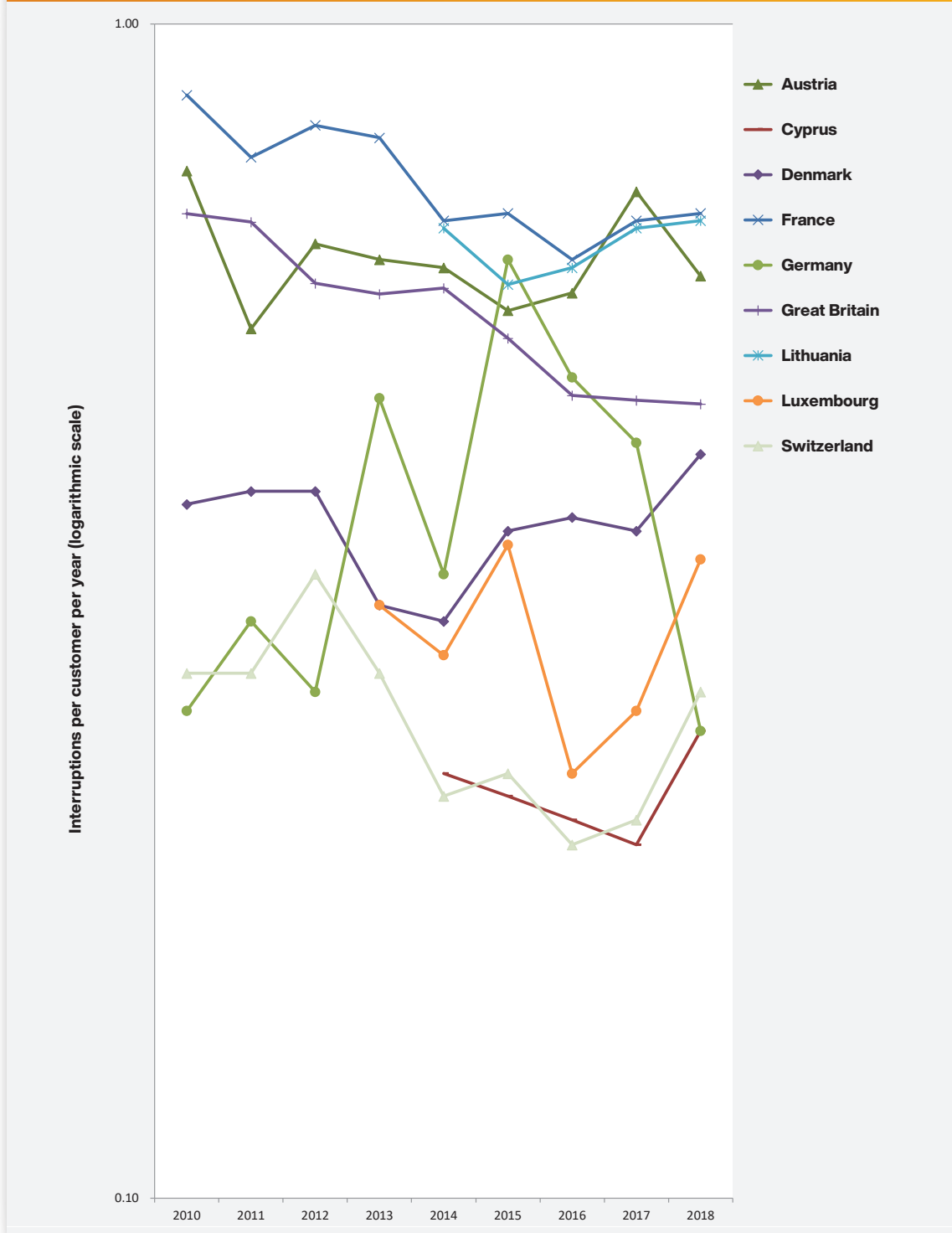
FIGURE 2-22: Unplanned long interruptions excluding exceptional events, SAIFI (interruptions per customer per year) – countries not exceeding one interruption in any of the years in the time series
