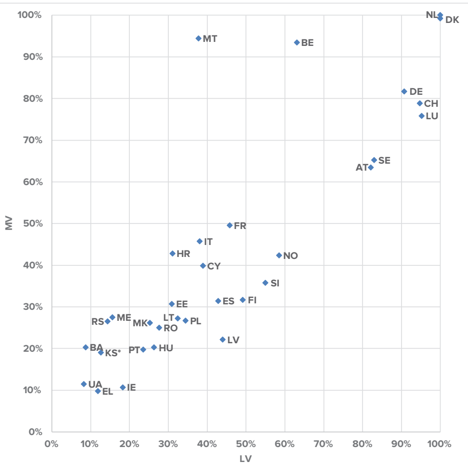
FIGURE 2-34: Percentage of LV and MV underground cables (2)
